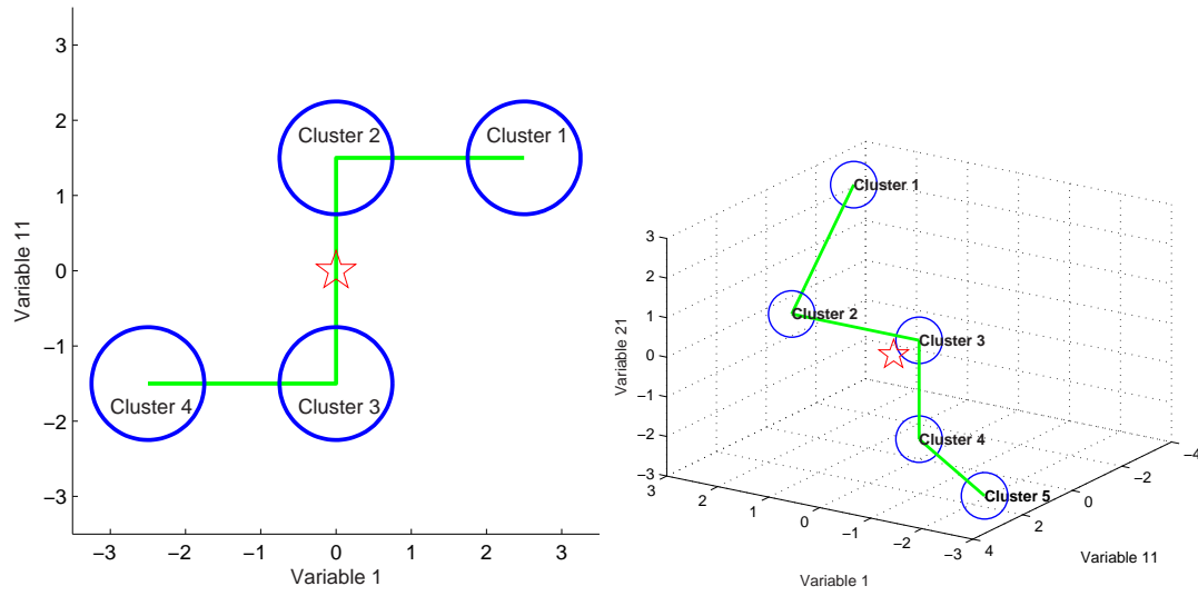
Figure 2. The distribution of informative variables in Simulation 1 (left) and Simulation 2 (right). The red star indicates the position of the overall sample mean.
