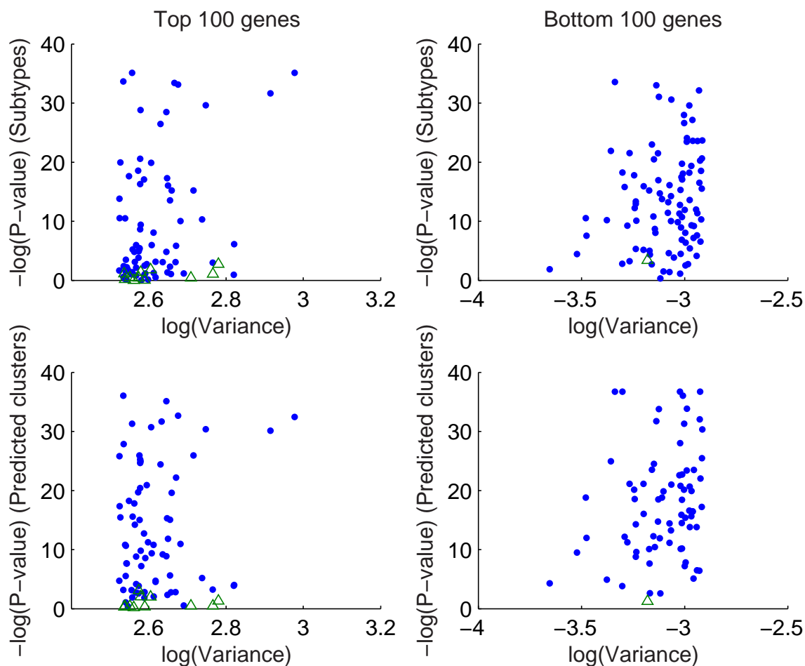
Figure 6. Plots of the negative logarithm p -values vs variance for PALL data. The left column is the top 100 genes (largest overall variances), and the right column is the bottom 100 genes. The upper row is negative logarithm p -values corresponding to an F -statistics comparing four tumor subtypes, and the lower row is the negative logarithm p -values for the six identified clusters. Triangles denote the genes that are not selected by the APFP method.
