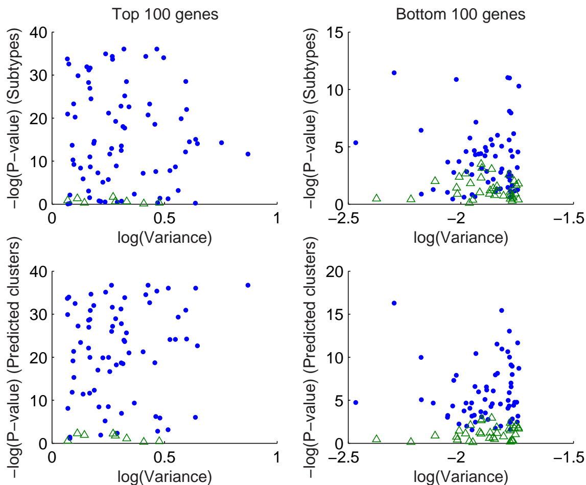
Figure 4. Plots of the negative logarithm p -values vs variance for SRBCT data. The left column is the top 100 genes (largest overall variances), and the right column is the bottom 100 genes. The upper row is negative logarithm p -values corresponding to an F -statistics comparing four tumor subtypes, and the lower row is the negative logarithm p -values for the six identified clusters. Triangles denote the genes that are not selected by the APFP method.
