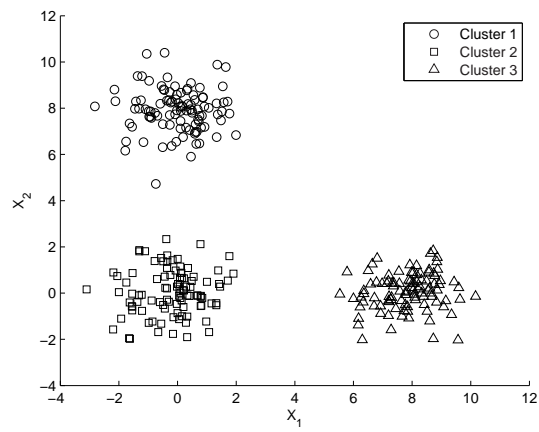
Figure 1. A toy example. Variable 1 is informative for separating clusters 2 and 3, and variable 2 is informative for separating clusters 1 and 2.
