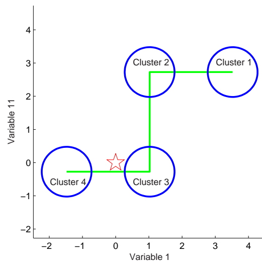
Figure 3. Simulation 3. The sample sizes of clusters 1, 2, 3 and 4 are 20, 20, 200, and 200, respectively. The red star indicates the position of the overall sample mean, and the plot is shifted to show centered data.
