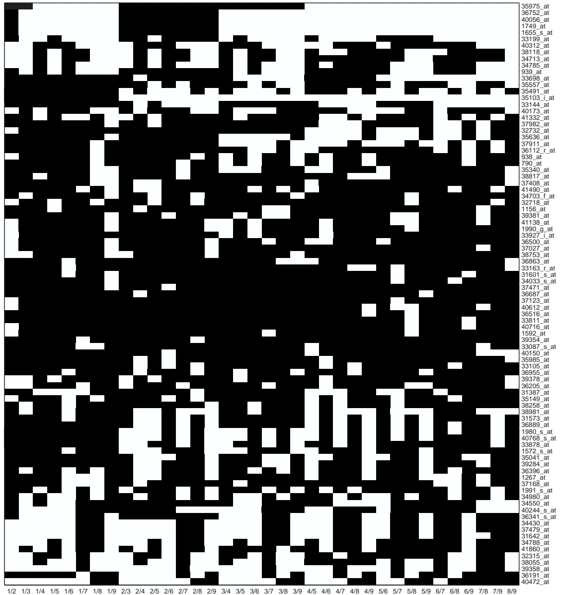
Figure 7. Pairwise variable selection results for the APFP method on the PALL data with top 100 genes. Each row corresponds to a gene. Each column corresponds to a cluster pair; for example, “1/2” indicates clusters 1 and 2. A black (white) spot indicates that the estimated means of the corresponding gene for the two clusters are different (the same).
