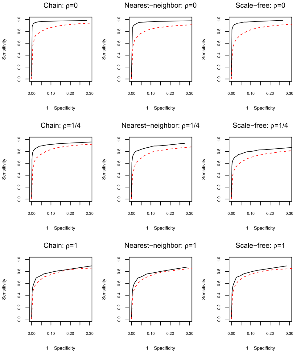
FIG. 3. Results for the balanced scenario ( n_1 = n_2 = n_3 = 300 ) and dimension p = 100 . Black solid curve: joint estimation; red dashed curve: separate estimation. The ROC curves are averaged over 10 replications. \rho is the ratio between the number of individual links and the number of common links.
