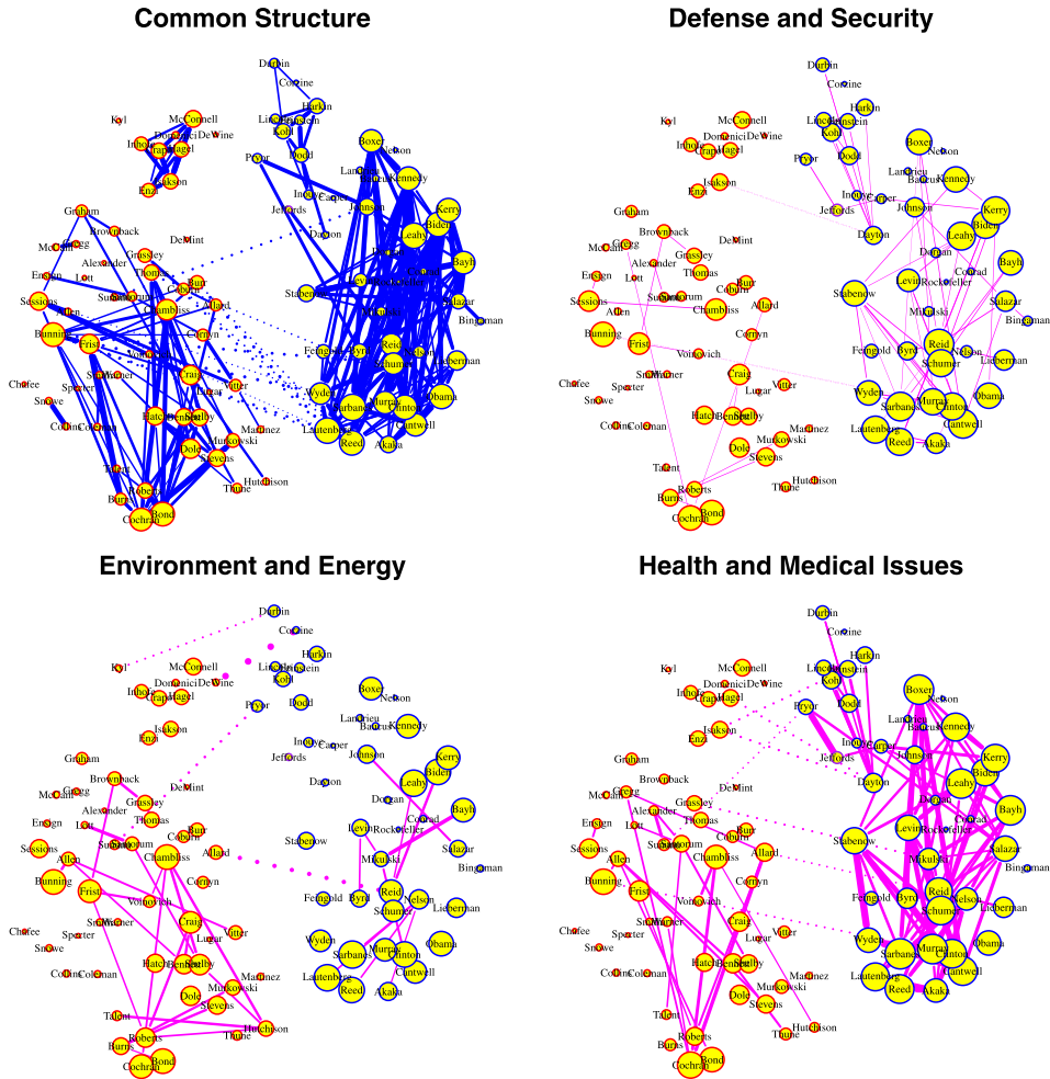
FIG. 5. The estimated graphical models for the three categories in the Senate voting data with an inclusion cutoff value of 0.4 and tuning parameter value of 0.5. Edges common to all three categories are shown under the heading “common structure”; all other edges are shown on category-specific graphs. The nodes represent the 100 senators, with red, blue and purple node colors corresponding to Republican, Democrat or Independent (Senator Jeffords), respectively. A solid line corresponds to a positive interaction effect and a dashed line to a negative interaction effect. The width of a link is proportional to the magnitude of the corresponding overall interaction effect.
