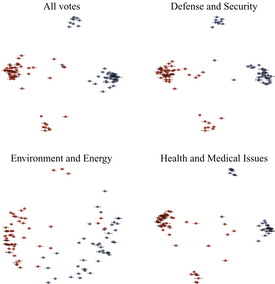
FIG. 6. Multidimensional scaling analysis for all the votes together, and the three individual categories. The nodes represent the 100 senators, with red, blue and purple node colors corresponding to Republican, Democrat or Independent (Senator Jeffords), respectively.
