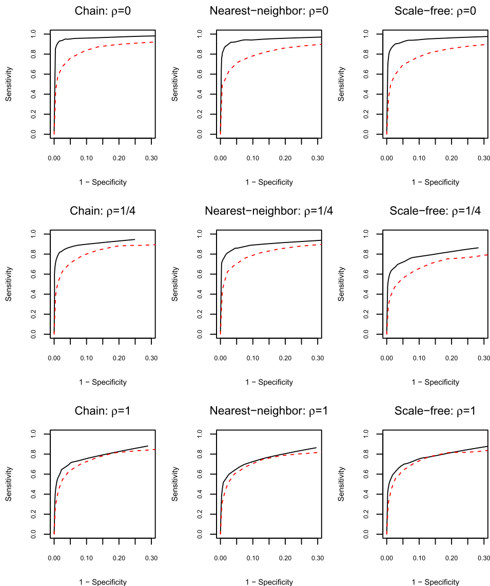
FIG. 4. Results for the unbalanced scenario ( n_1 = 200 , n_2 = 300 , n_3 = 400 ) and dimension p = 100 . Black solid curve: joint estimation; red dashed curve: separate estimation. The ROC curves are averaged over 10 replications. \rho is the ratio between the number of individual links and the number of common links.
