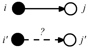
Figure 1: Pair similarity for directed networks
