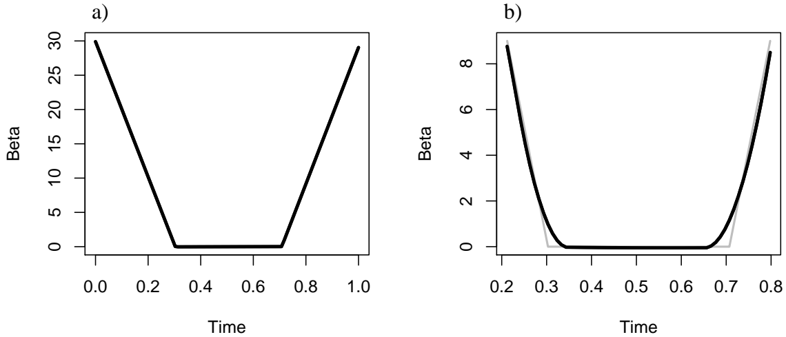
Figure 2: Plots of true beta curve (grey) and corresponding FLiRTI estimates (black). For each plot we constrained a) zeroth and second derivative, b) zeroth and third derivative.
