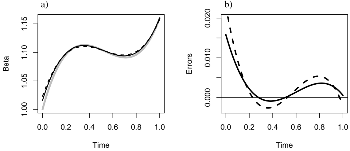
Figure 3: a) True beta curve (grey) generated from a cubic curve. The FLiRTI estimate from constraining the zeroth and fourth derivative is represented by the solid black line and the B-spline estimate is the dashed line. b) Estimation errors using the B-spline method (dashed) and FLiRTI (solid).
