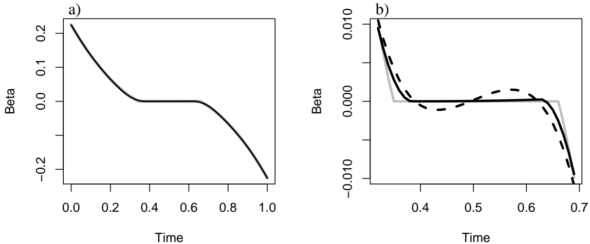
Figure 1: a) True beta curve (grey) generated from two quadratic curves and a section with \beta(t) = 0 . The FLiRTI estimate from constraining the zeroth and third derivative is shown in black. b) Same plot for the region 0.3 \leq t \leq 0.7 . The dashed line is the best B-spline fit.
