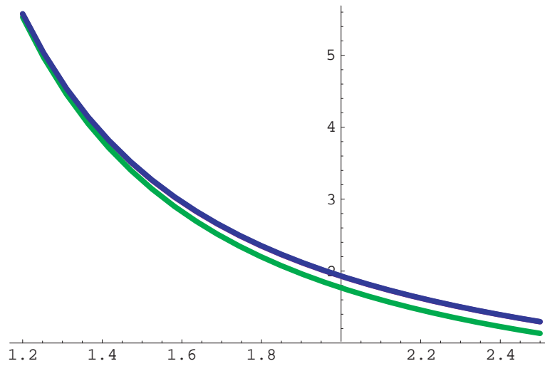
Figure 3.1: Information bounds, \alpha = 3 , 1.2 \leq \beta \leq 2.5 ; green = I^{-1}(P|\nu, \mathcal{P}_0) , purple = I^{-1}(P|\nu, \mathcal{P}) , blue = Var_{\theta}(X) ; (purple coincides with blue so not visible!)
